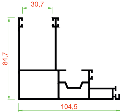
TG-103 YAN KASA (ALT) 1.169 KG/M
